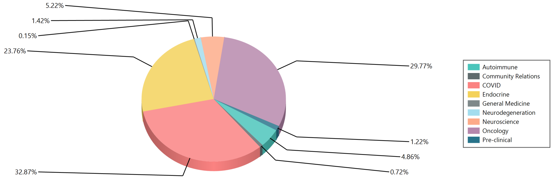
Program Category
